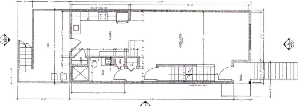
1 FIRST FLOOR PLAN SCALE: 1/8"=1'-0"
